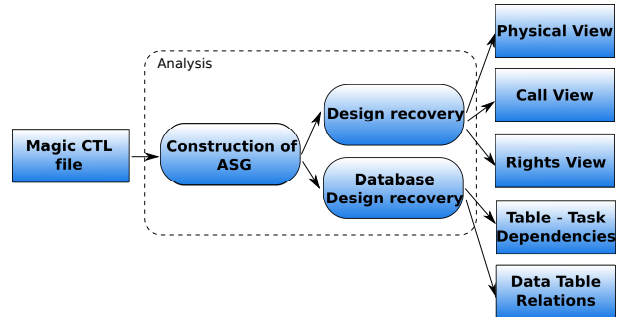
Figure 1. Overview of the design recovery process.
